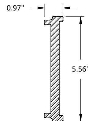
31 ALUMINUM REINFORCEMENT
