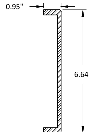
32 ALUMINUM REINFORCEMENT
