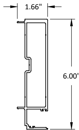
16 MALE MULLION
