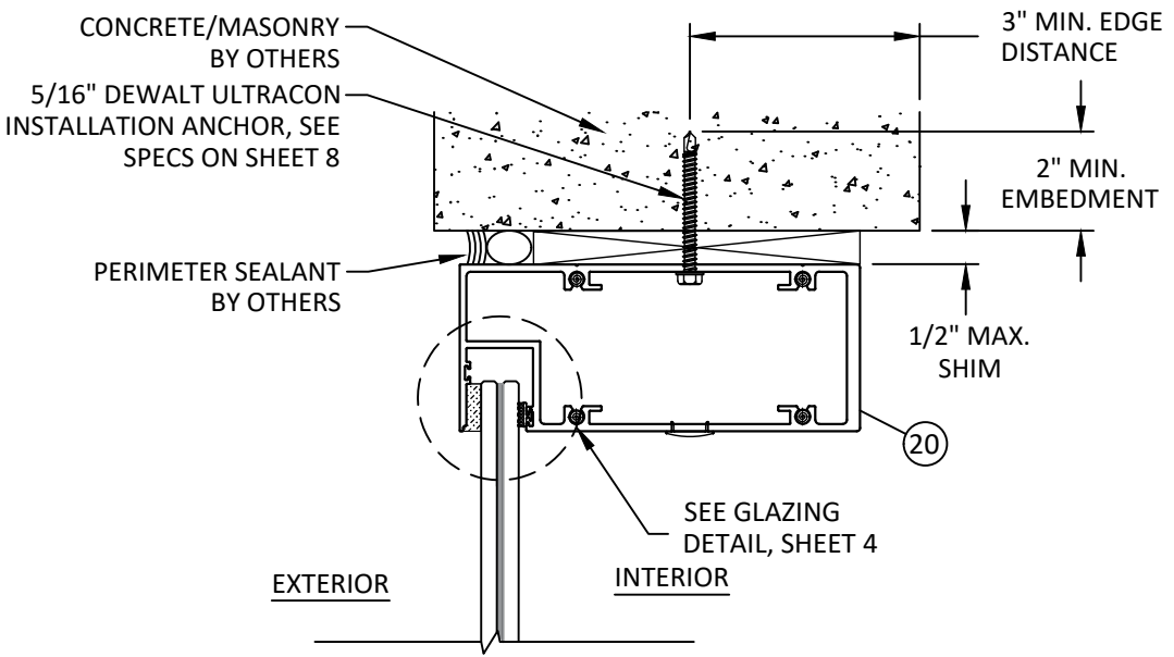
F 11 VERTICAL SECTION HEAD - CONCRETE/MASONRY SUBSTRATE
