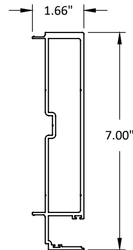
18 MALE MULLION
