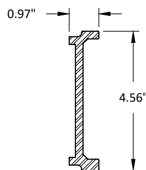
29 ALUMINUM REINFORCEMENT
