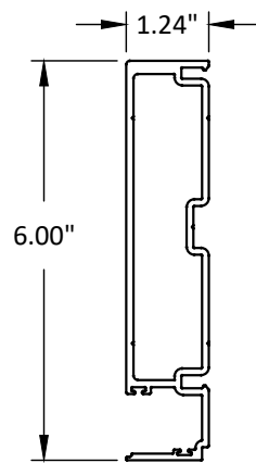
15 FEMALE MULLION
