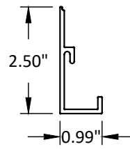
6 GLASS STOP
